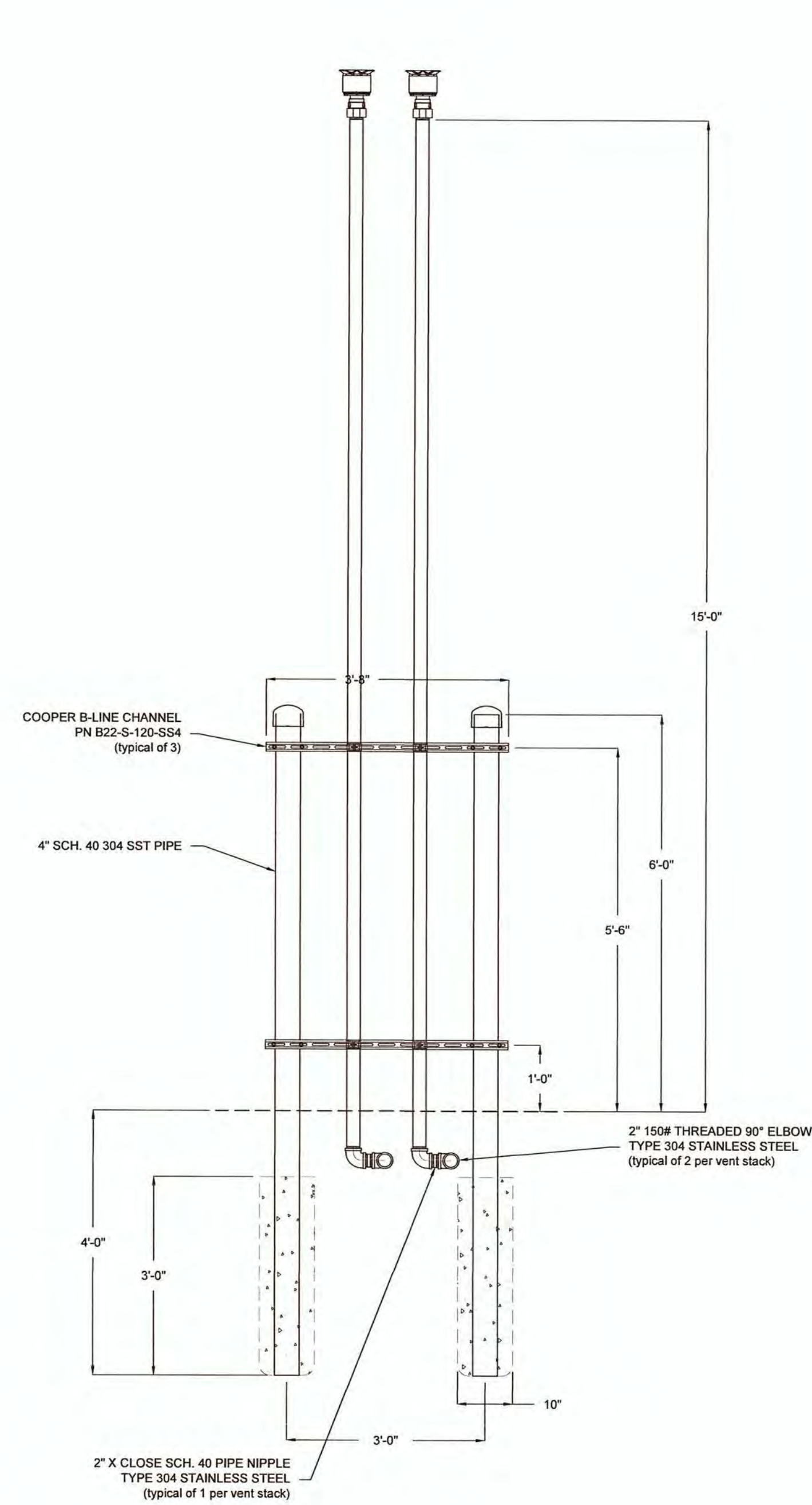
FRONT VIEW
