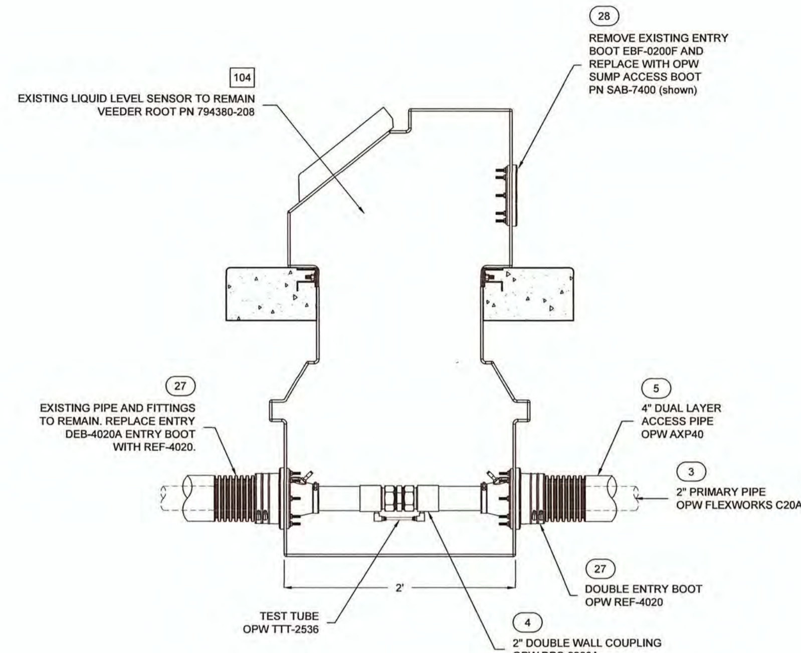
ELEVATION TYPICAL FOR TWO TRANSITION SUMPS.
