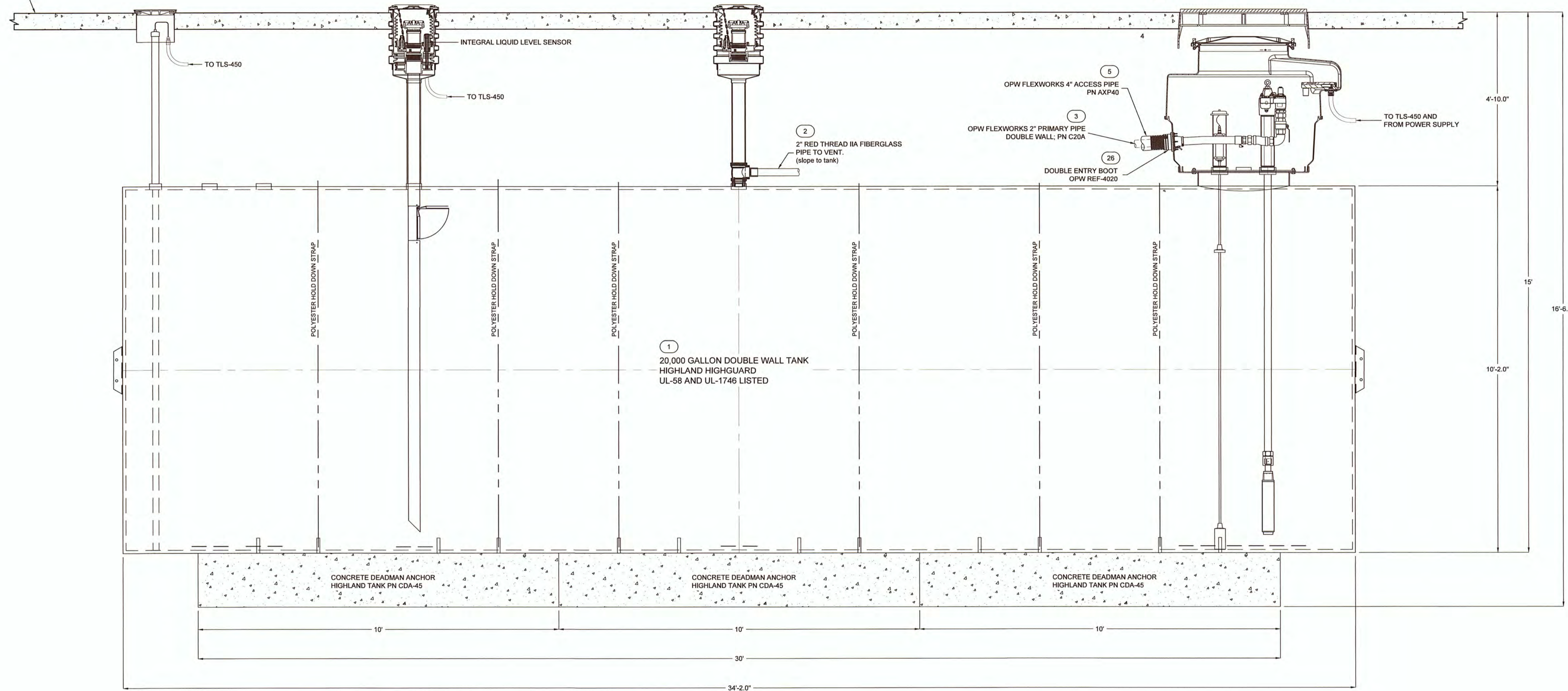
ELEVATION VIEW
