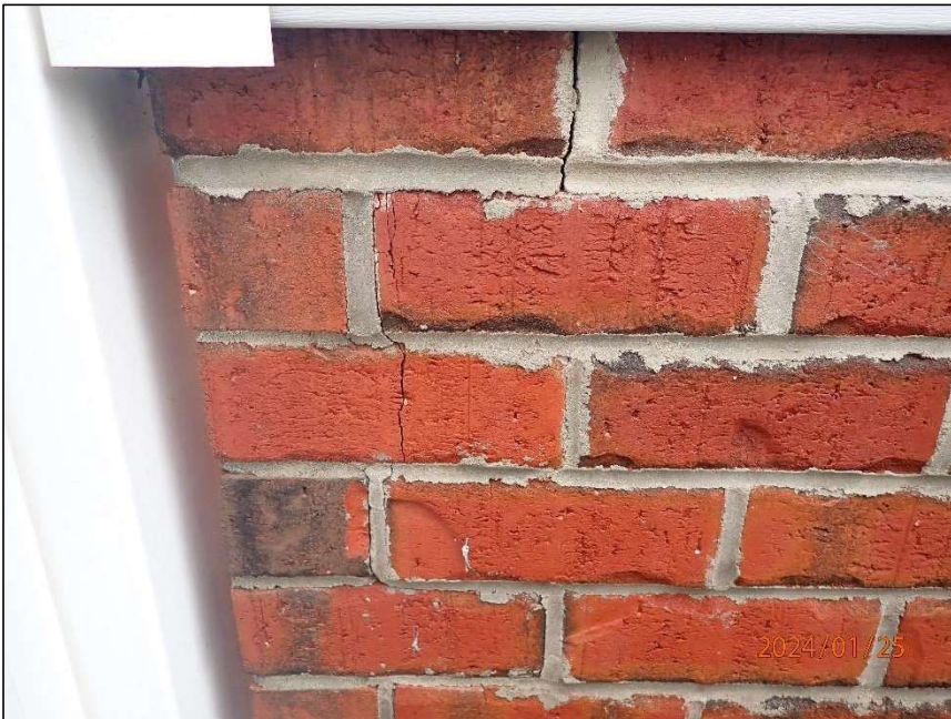
Photo 10 Step and vertical crack
