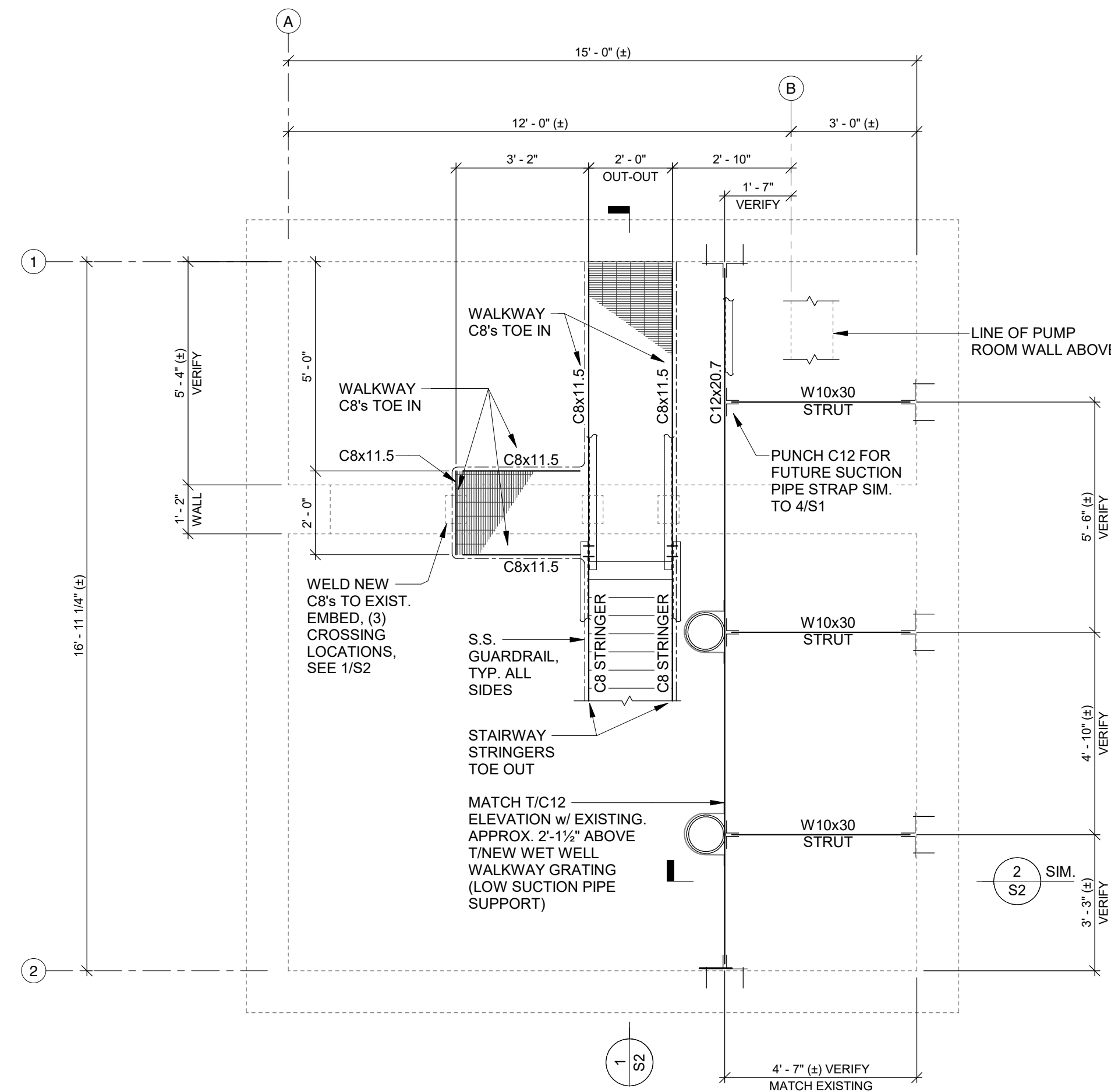
WET WELL AT CATWALK 2 3/8" = 1'-0" S1
