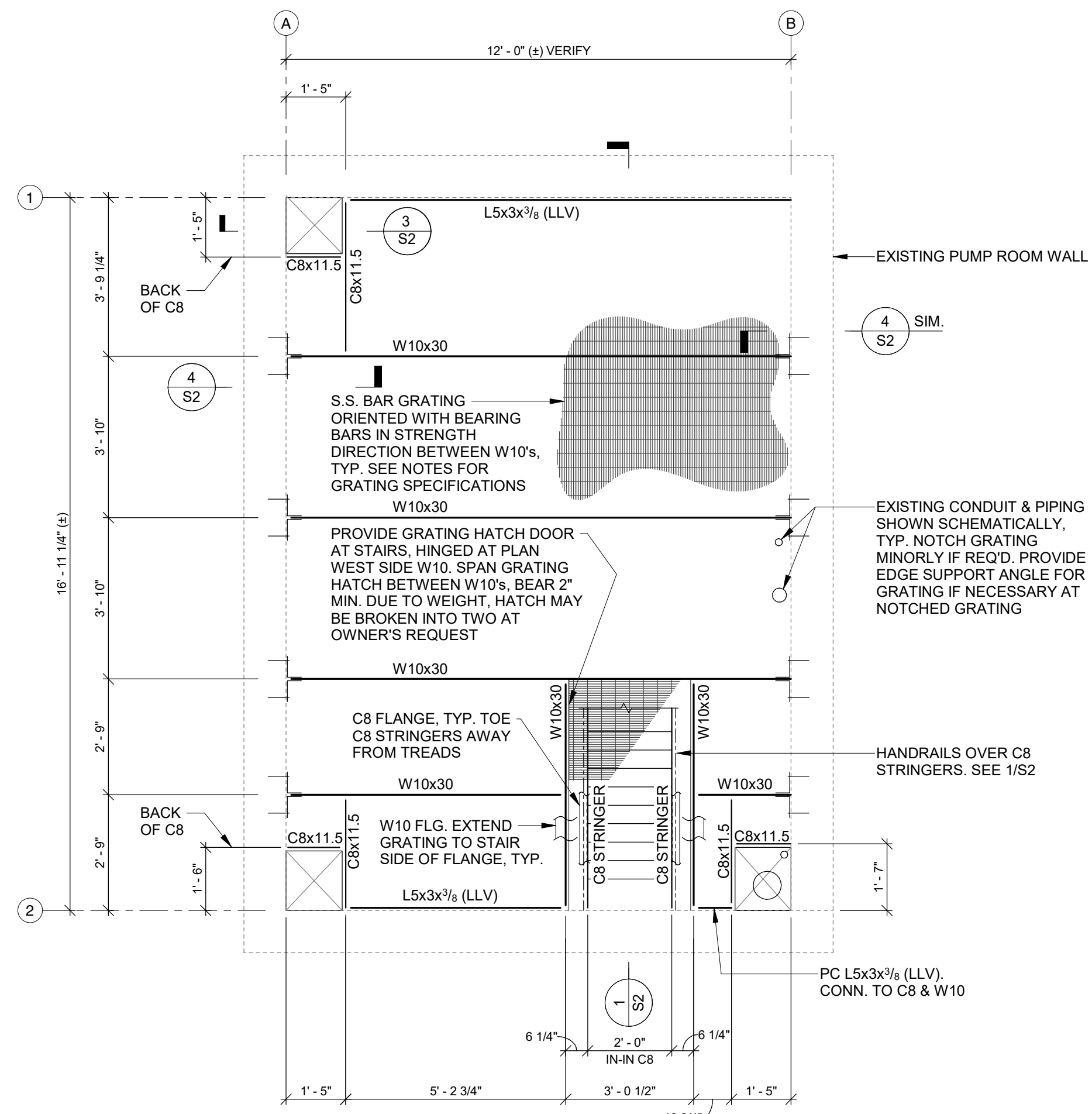
TOP OF WET WELL 1 3/8" = 1'-0" S1
